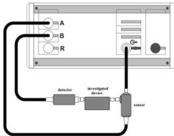
Figure 7. Scheme of measurement of transmission and reflection coefficients modules.
