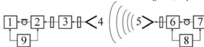
Figure 4. Block diagram of the experimental determination of orientation diagram: 1-indicator device; 2-receiver block; 3-adjustable attenuator; 4- receiver megaphone; 5- transmitter megaphone; 6-generator block; 7-modulated block; 8, 9-power supply.
