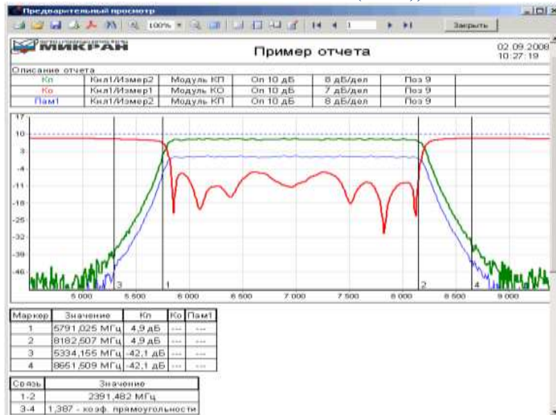
Figure 9. Results of modules of transmission and reflection coefficients obtained from computer.
